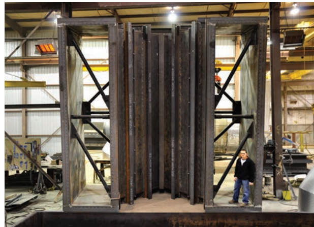
Bifurcated duct section, approximately 18' x 16' Corten.
