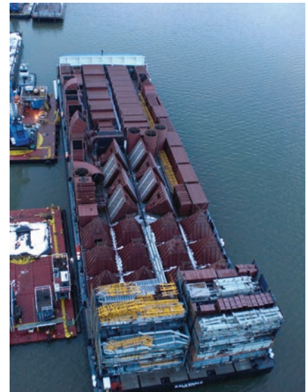
2.5 million pounds of duct, structural steel, modular baghouses & platforms fabricated by Danser & shipped to HI.
