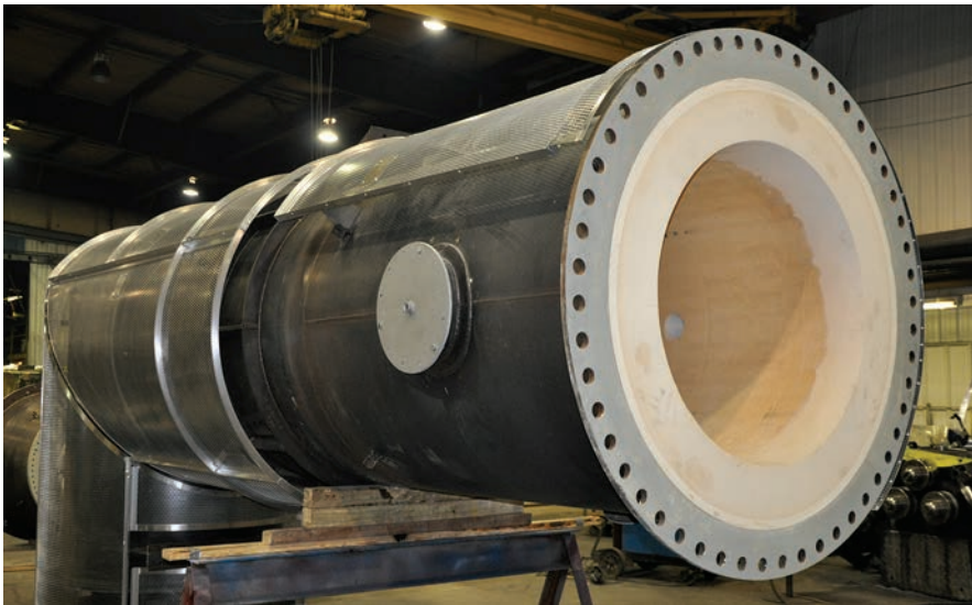
Flue gas system with 2300° F Vacuct® insulation, 36" ID x 48" OD carbon steel duct with SS expanded metal protective shield.
